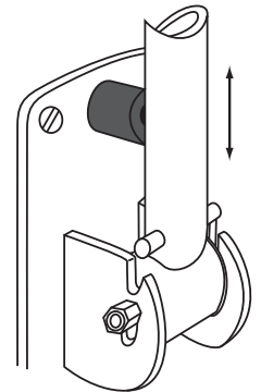
Detail of Grab Bar Locking Mechanism
